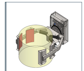
Electric rotation clamp
